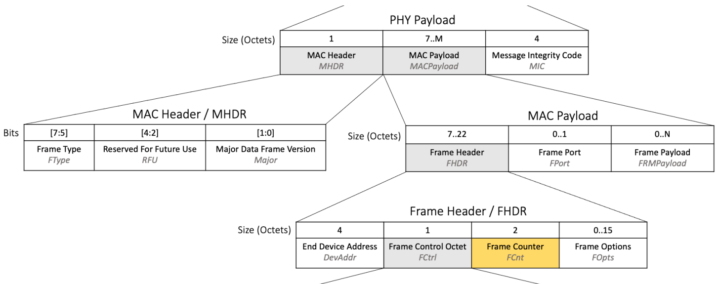
Figure 14. FCnt field highlighted in the LoRaWAN downlink packet structure
