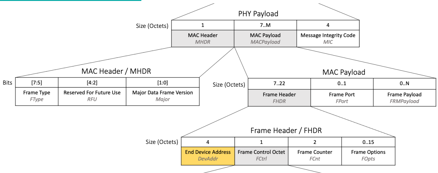
Figure 11. DevAddr field highlighted in the LoRaWAN downlink packet structure
