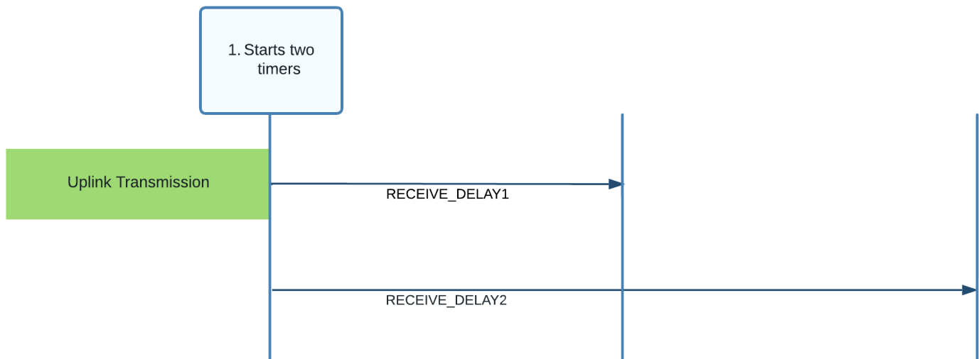
Figure 6. RECEIVE_DELAY1 and RECEIVE_DELAY2 started following uplink transmission
