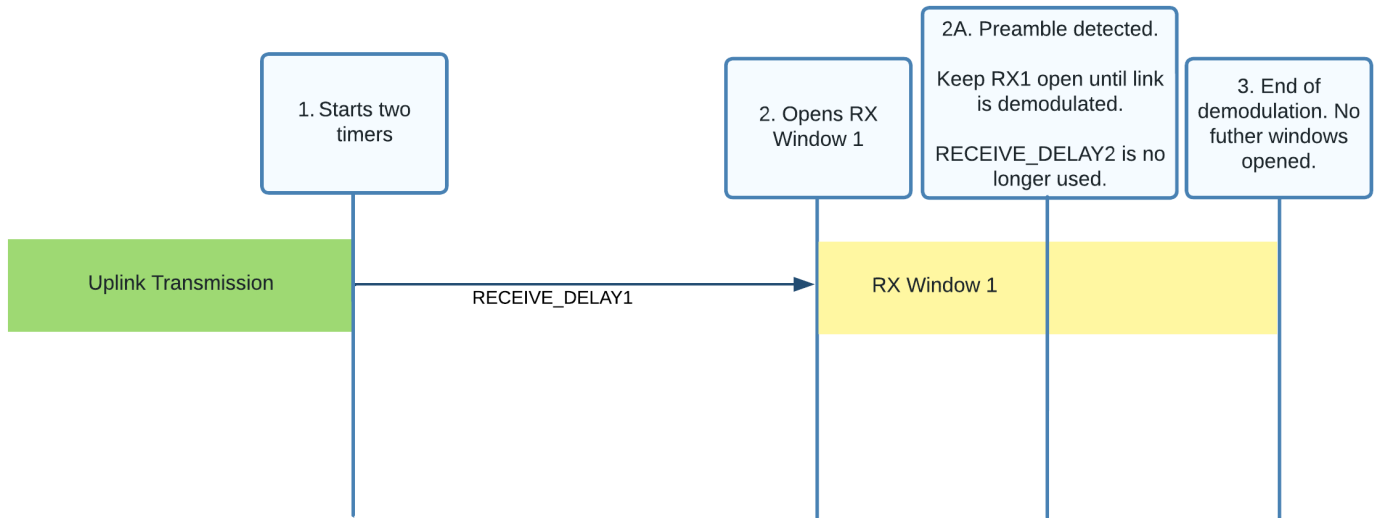
Figure 8. Preamble detected in the first receive window (RX1)
