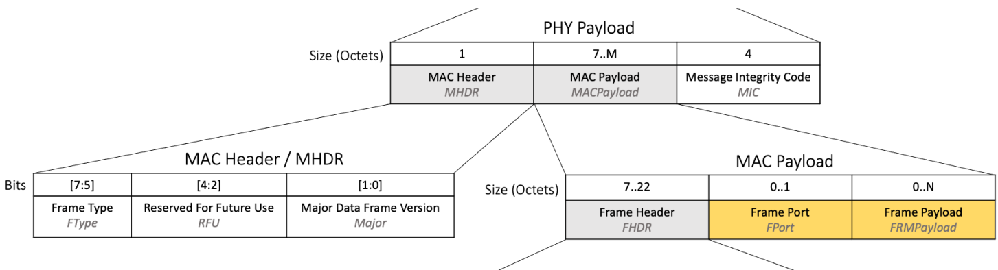
Figure 17. FPort and FRMPayload fields highlighted in the LoRaWAN downlink packet structure
