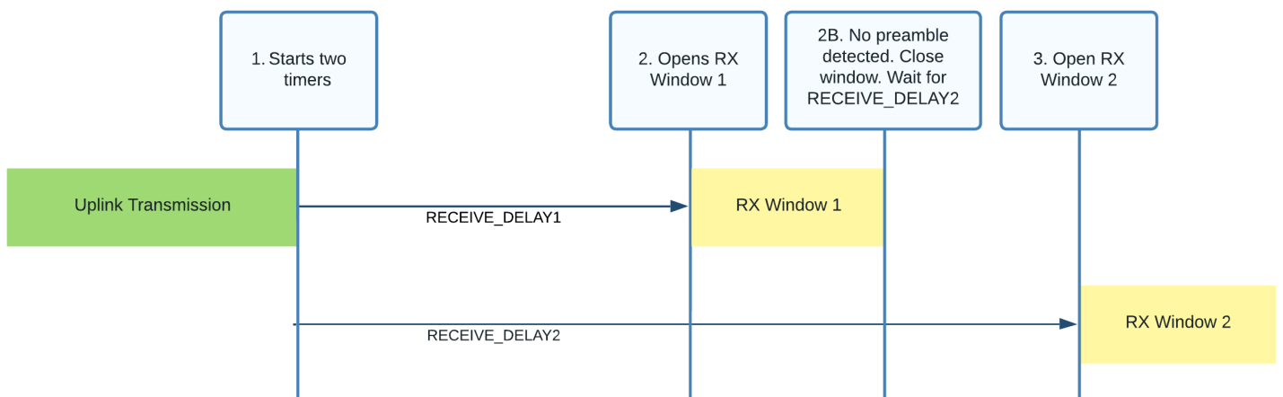
Figure 9. Opening the second receive window (RX2)
