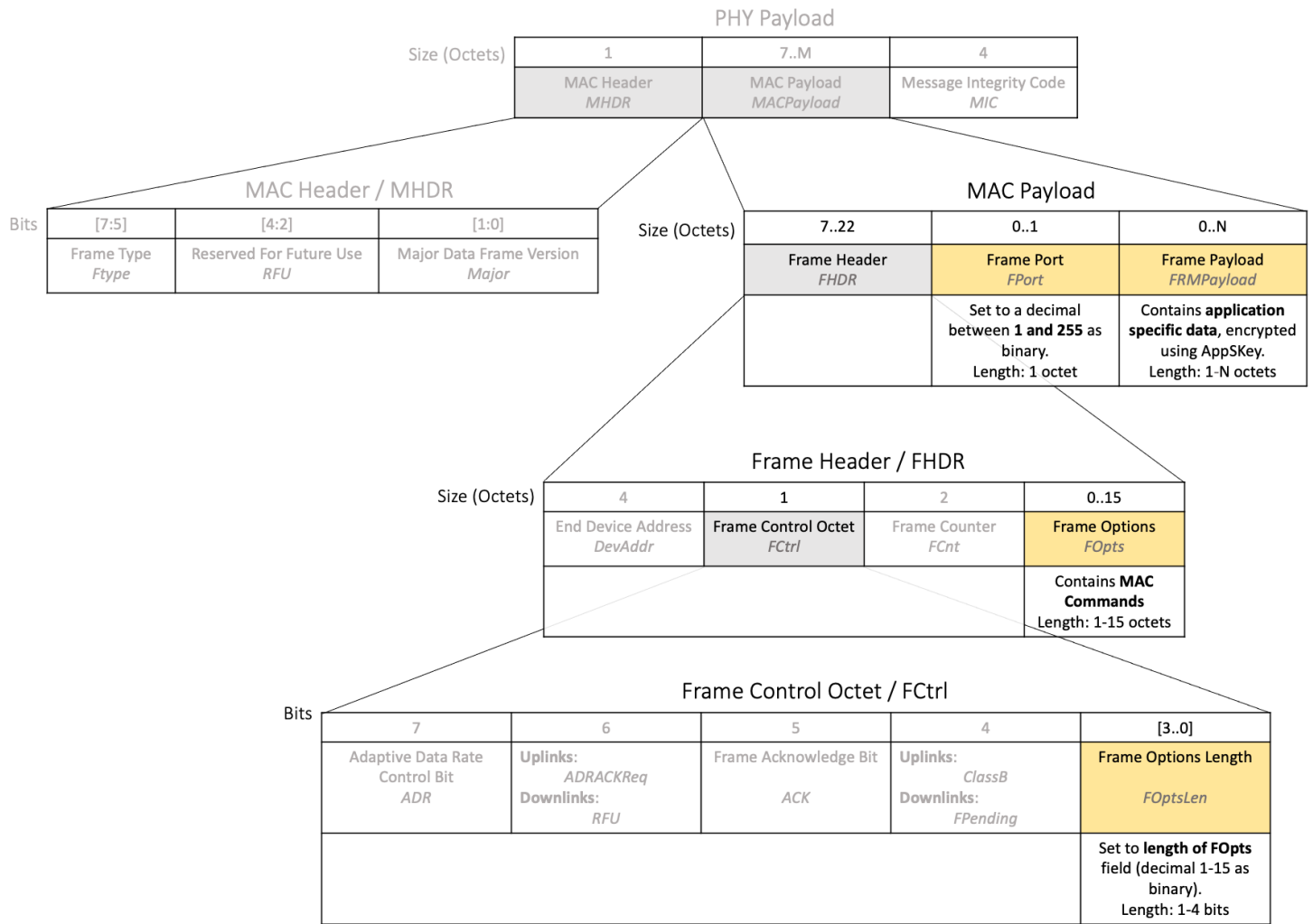
Figure 20. Use of FPort , FRMPayload , FOpts , and FOptsLen fields when sending MAC commands as well as application data
