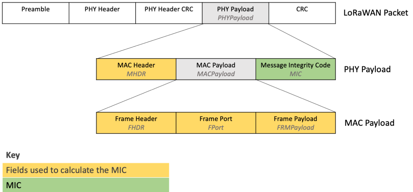
Figure 5. Fields used to calculate the MIC
