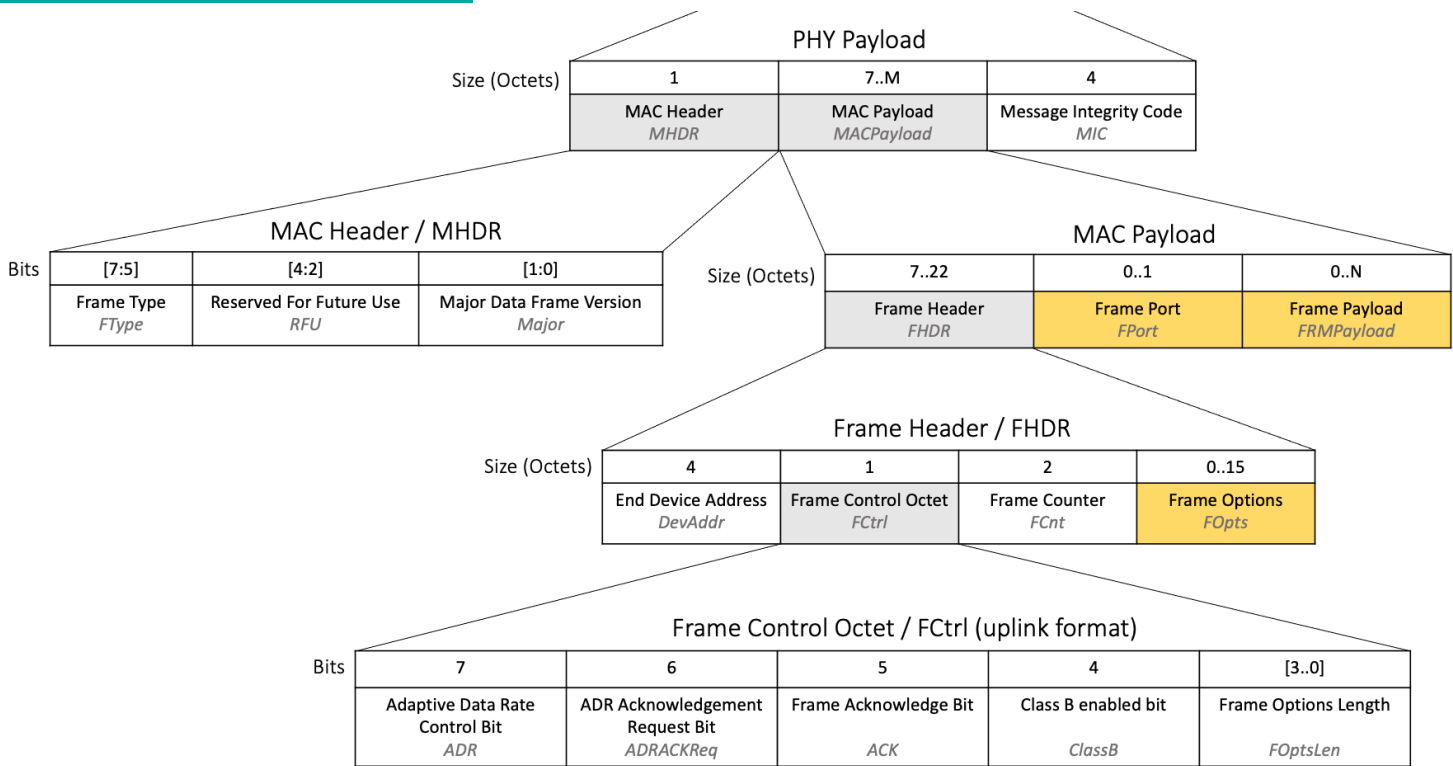
Figure 3. Application data and MAC command fields highlighted in a LoRaWAN uplink packet
