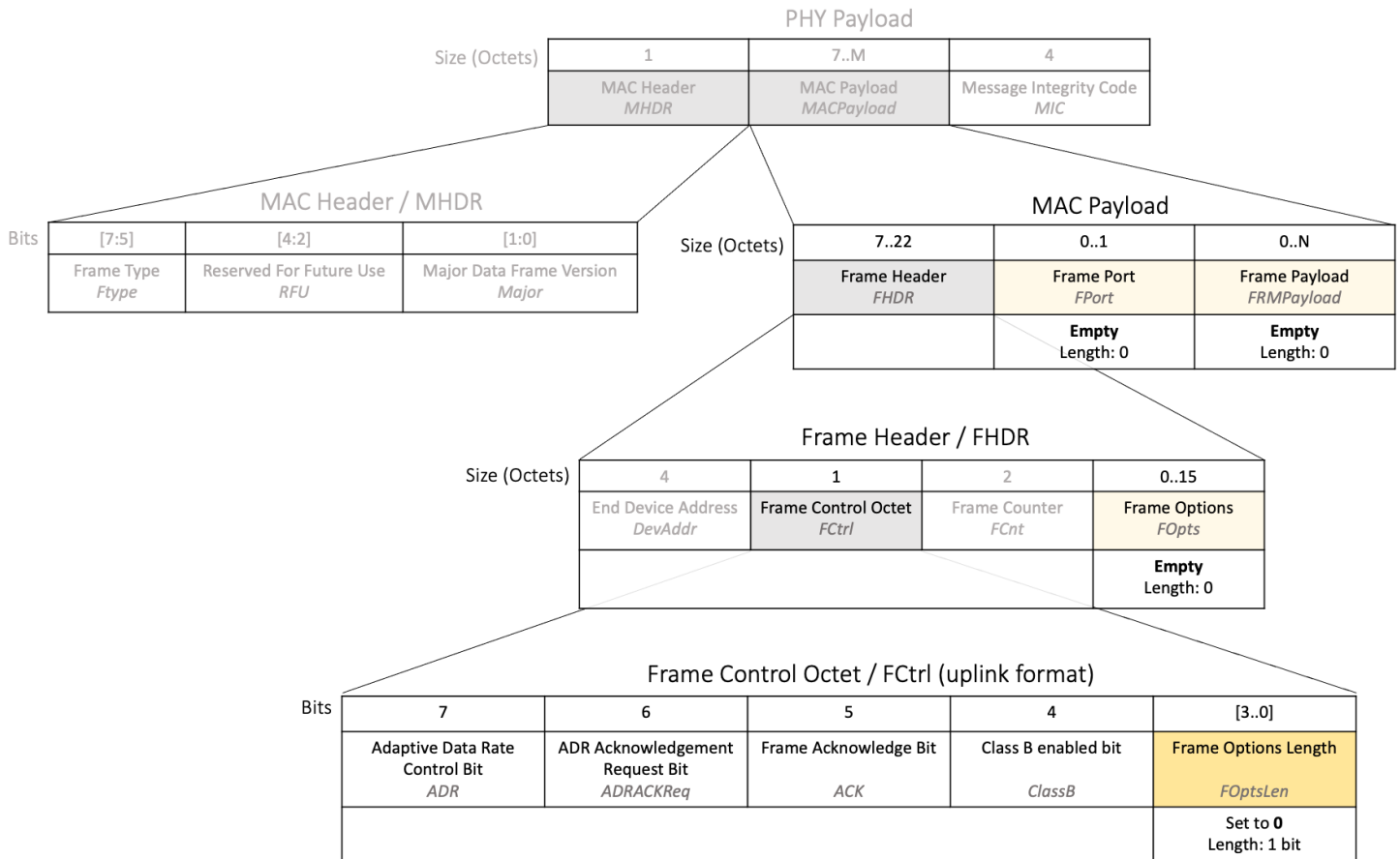
Figure 21. Use of FPort , FRMPayload , FOpts , and FOptsLen fields when sending an empty message
