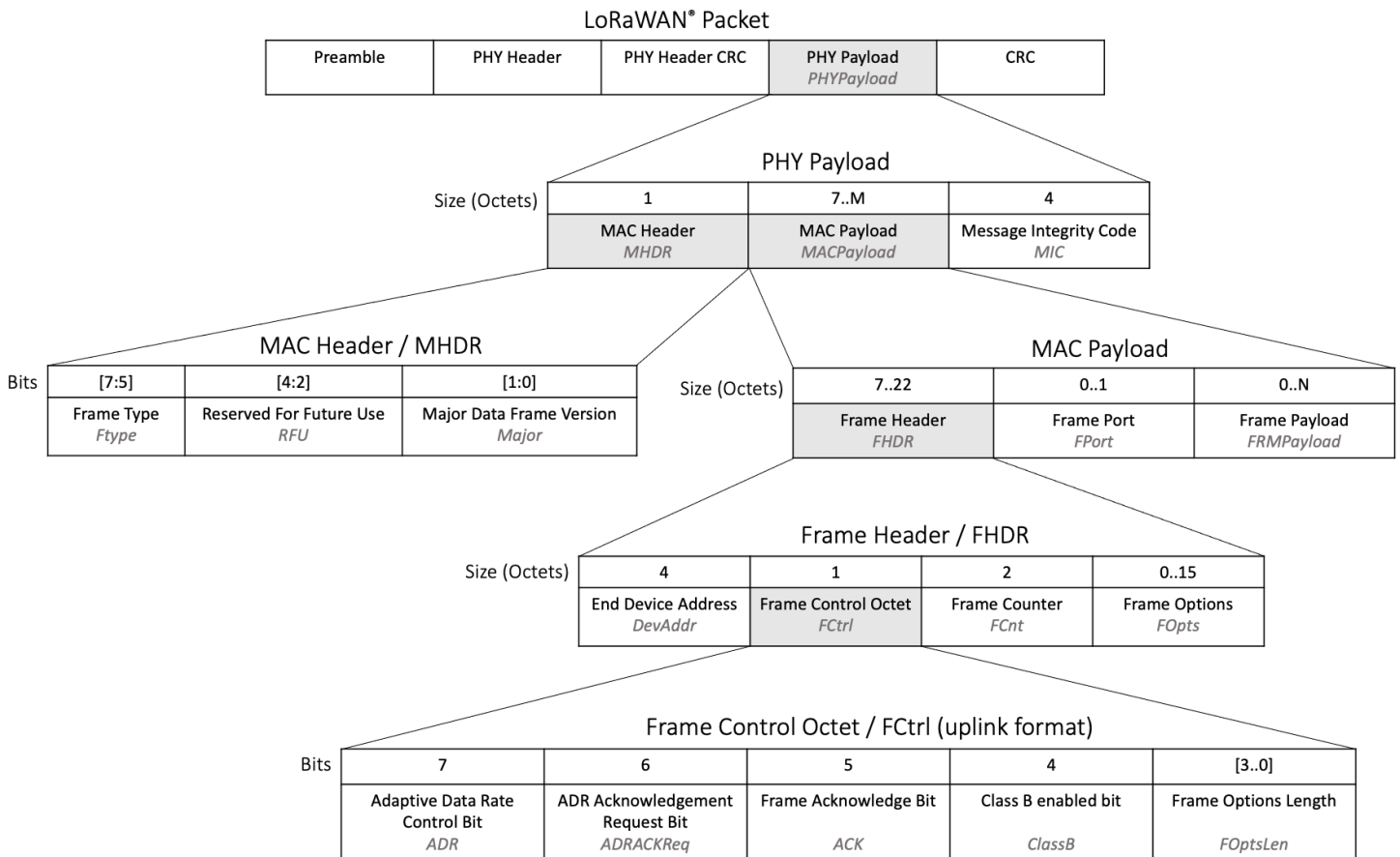
Figure 1. Fields contained in a LoRaWAN uplink
