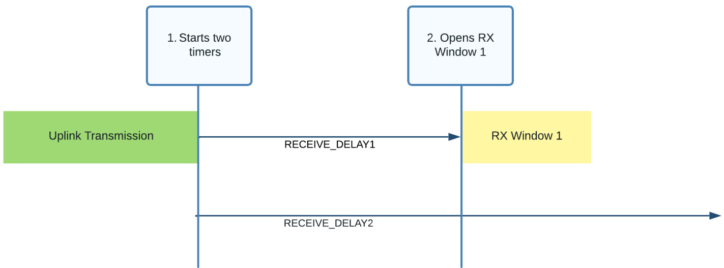
Figure 7. RX Window 1 opened following RECEIVE_DELAY1
