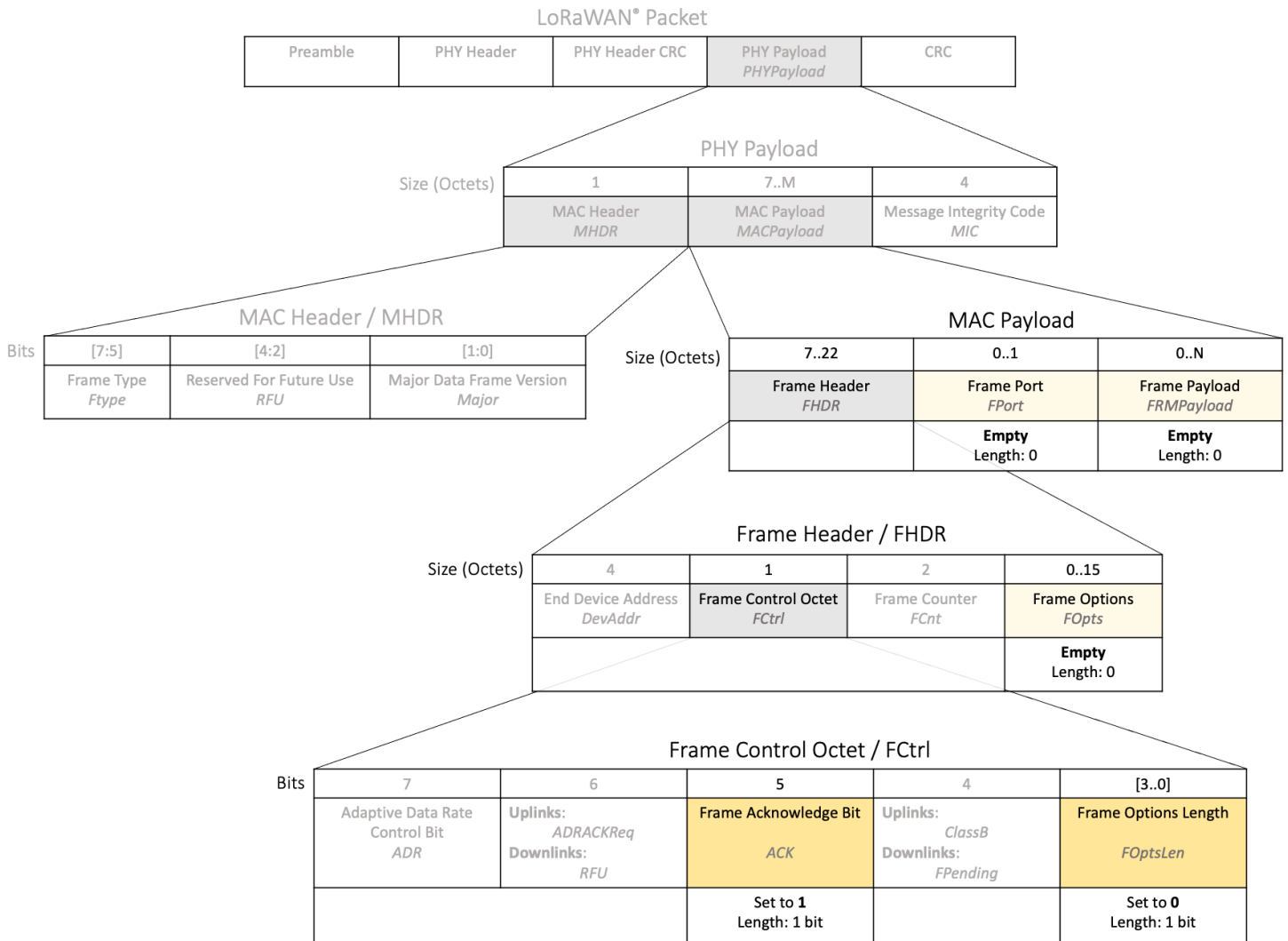
Figure 22. Use of FPort , FRMPayload , FOpts , FOptsLen , and ACK fields when sending a confirmed downlink acknowledgement or receiving a confirmed uplink acknowledgement
