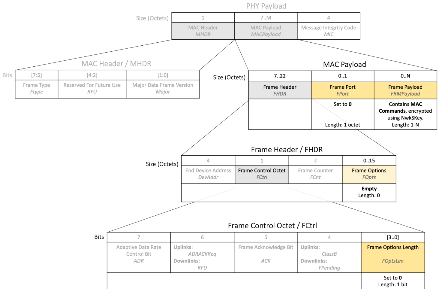
Figure 19. Use of FPort , FRMPayload , FOpts , and FOptsLen fields when sending MAC commands only
