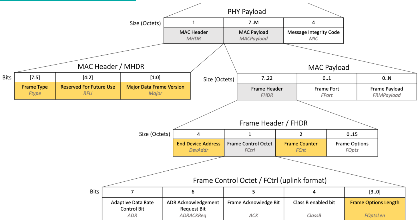
Figure 2. Metadata fields highlighted in a LoRaWAN uplink
