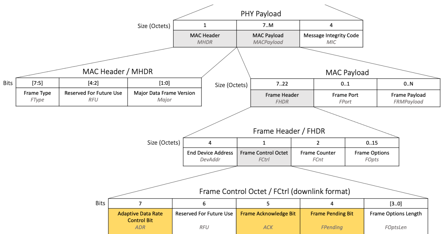
Figure 15. Bit fields highlighted in the LoRaWAN downlink packet structure
