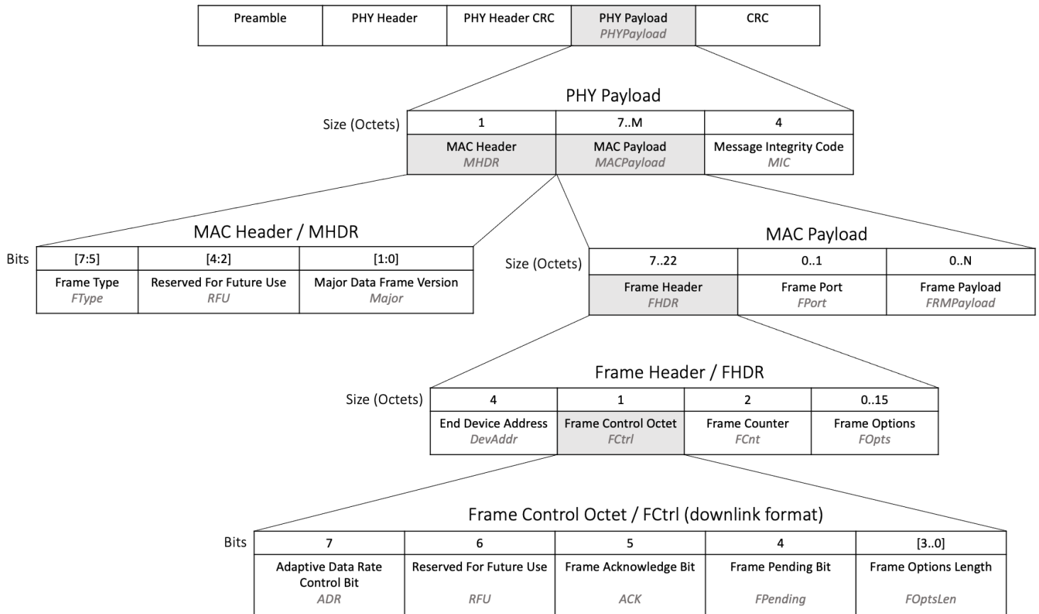
Figure 10. Fields contained in a LoRaWAN downlink packet
