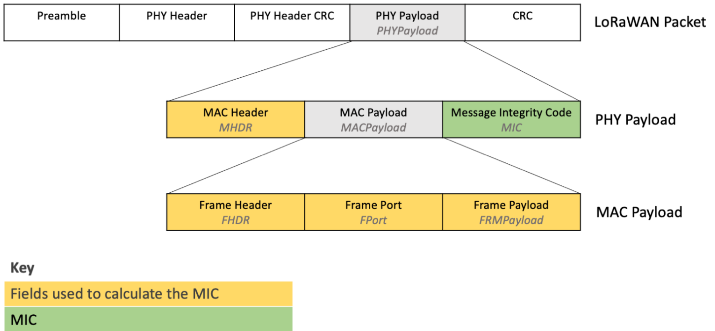
Figure 13. Fields used to calculate the MIC
